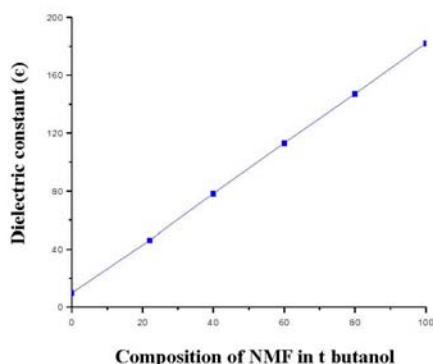
Fig. 1 Graph for the estimation of dielectric constant of various NMF-t-butanol mixtures at 25°C.
