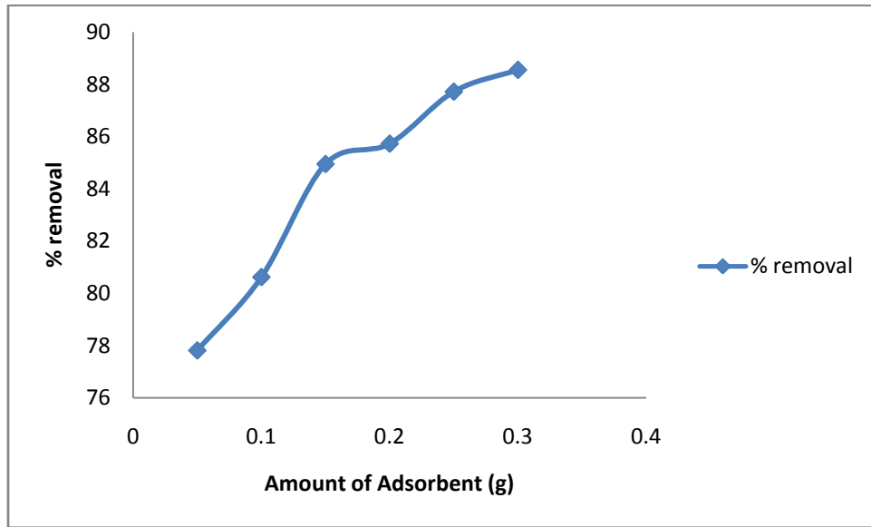
Fig. 2 Effect of Adsorbent dose (% removal)
