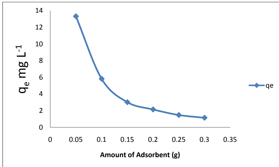
Fig 3 Effect of Adsorbent dose ( q_e )
